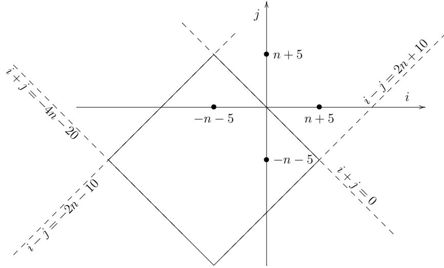
Figure 1: Problem domain
